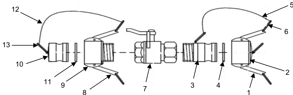
Figure 1. Filler/Discharge Ball Valve.
