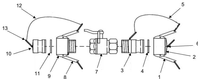
Figure 1. Tank or Berm Liner Drain Ball Valve.
