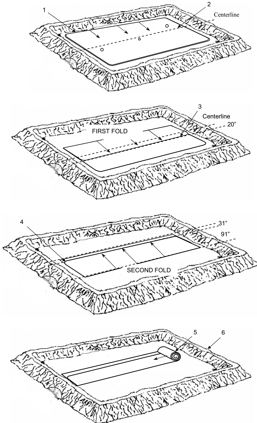
Figure 13. Tank Envelope Folding Procedures.
