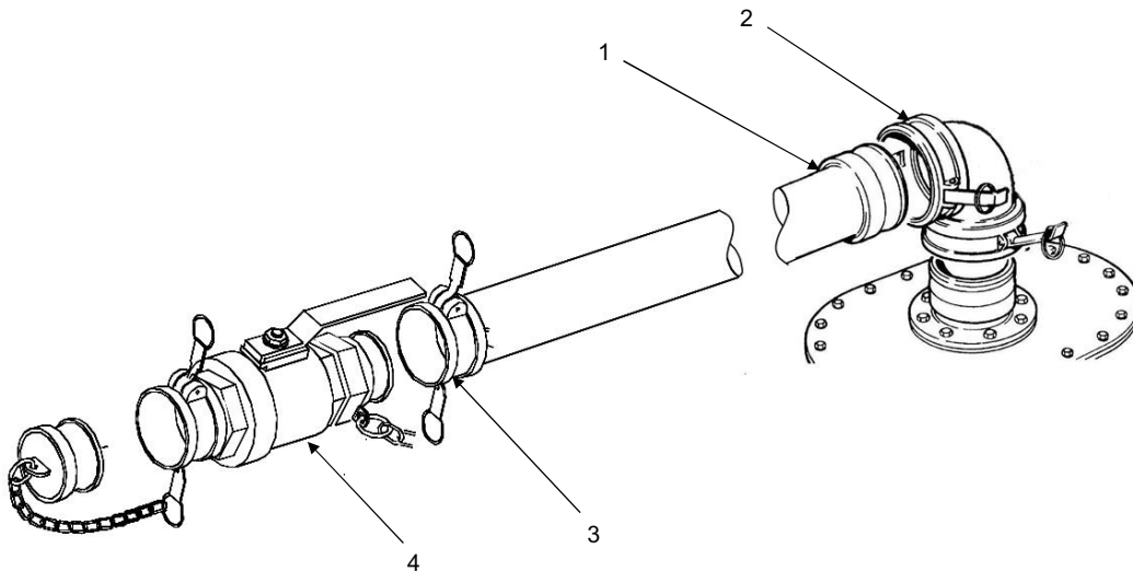
Figure 10. Filler/Discharge Hose Assembly and Filler/Discharge Valve.
