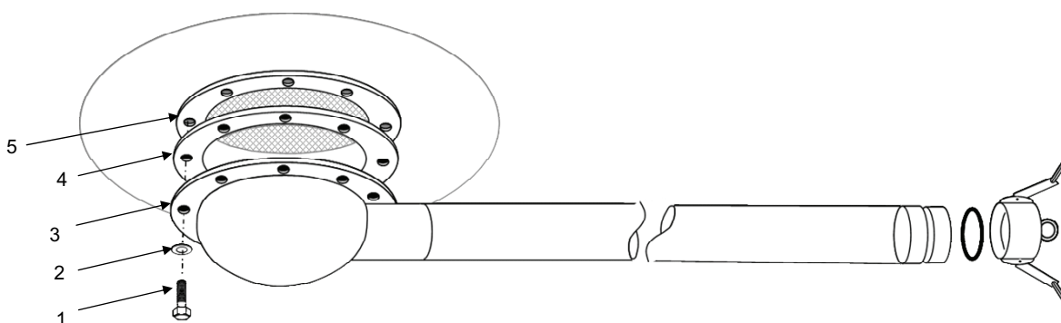
Figure 1. Tank Drain Hose Assembly, Bowl x Cam.
