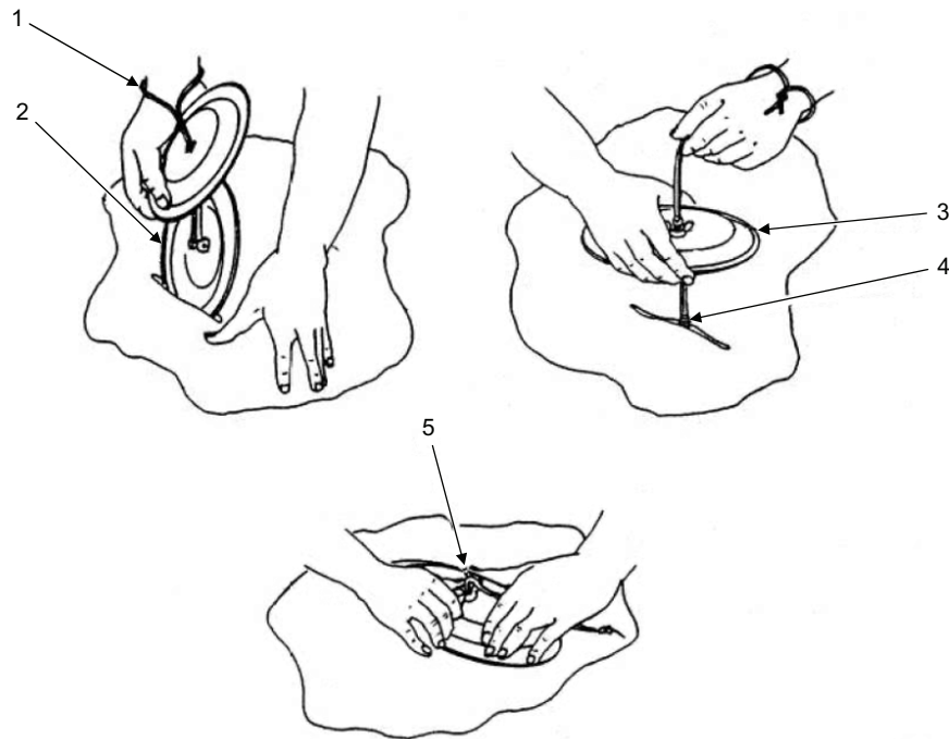
Figure 3. Mechanical Patch Installation.
