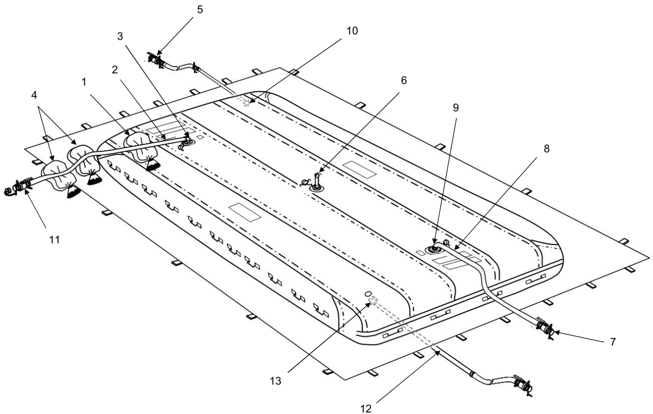
Figure 11. Elevated Connections.
