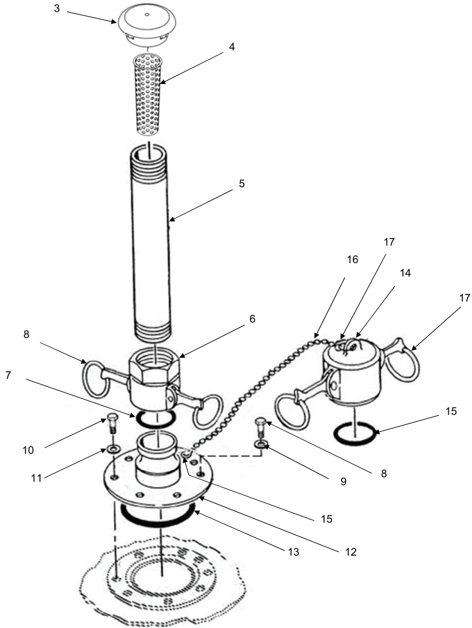
Figure 7. Vent Port Assembly.
