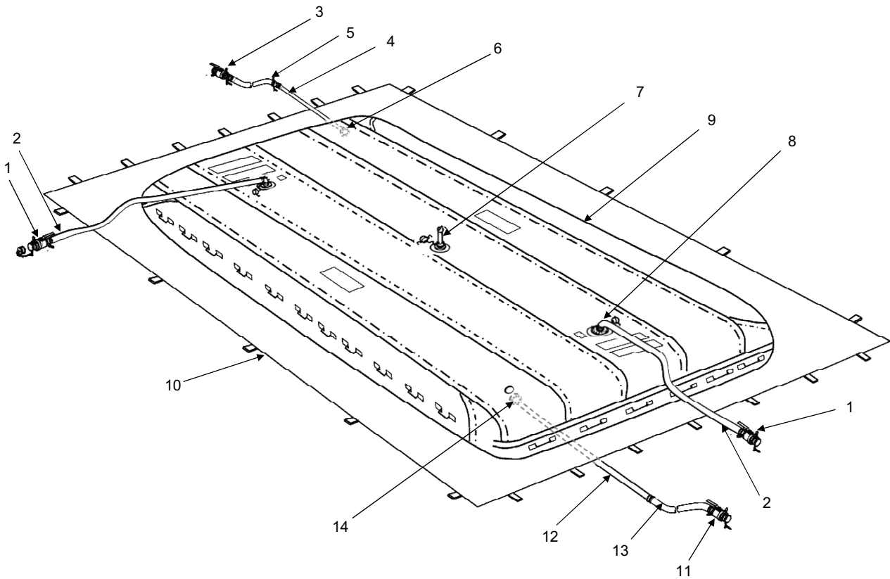
Figure 1. 50,000 Gallon Fuel Storage Collapsible Fabric Tank Assembly.
