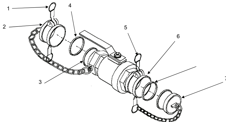
Figure 1. Filler/Discharge Ball Valve Assembly.
