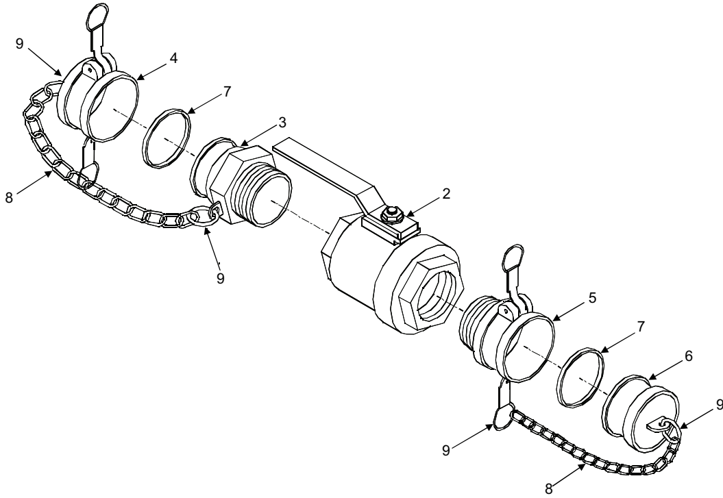
Figure 2. Filler/Discharge Ball Valve Assembly.
