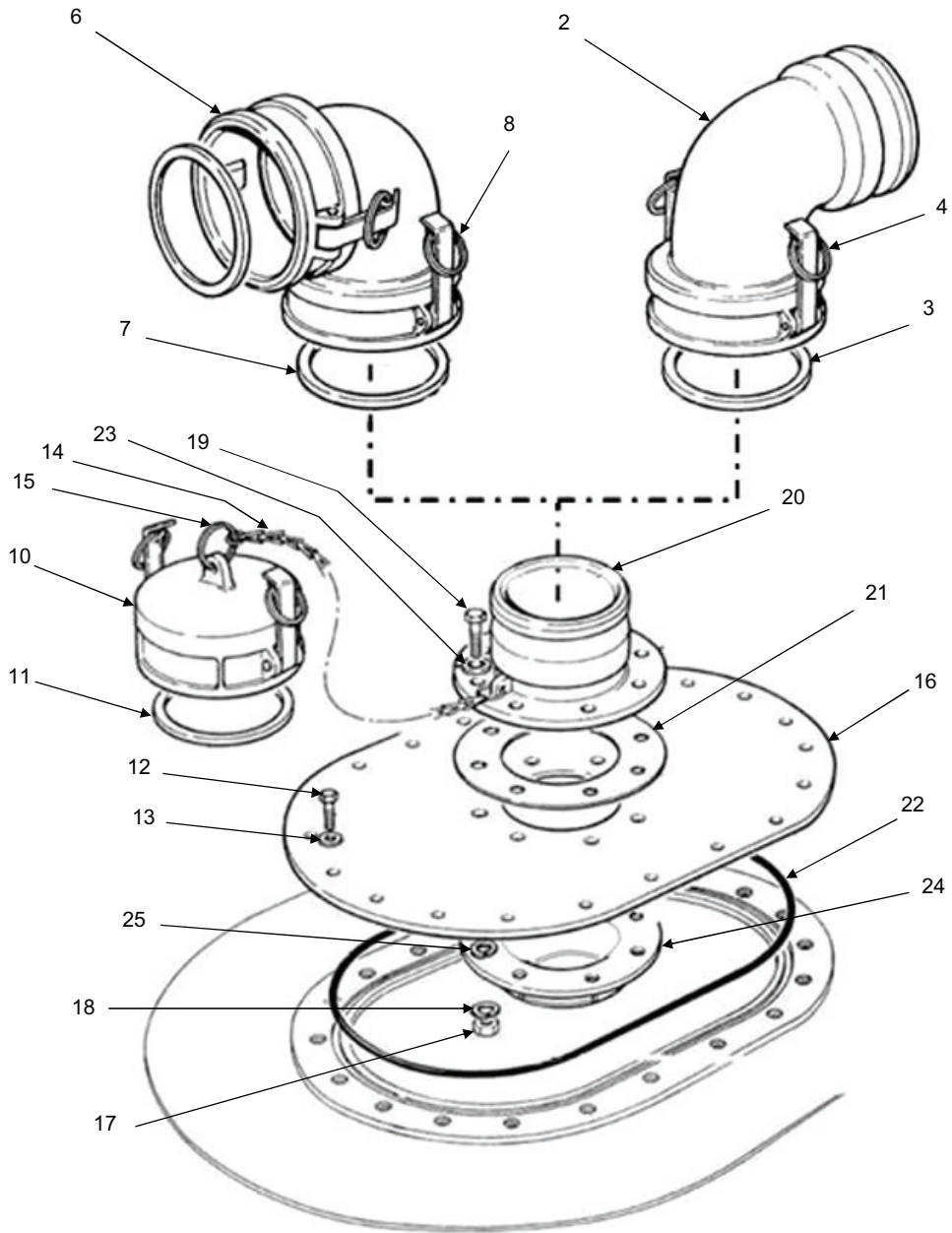
Figure 8. Filler/Discharge Assembly.
