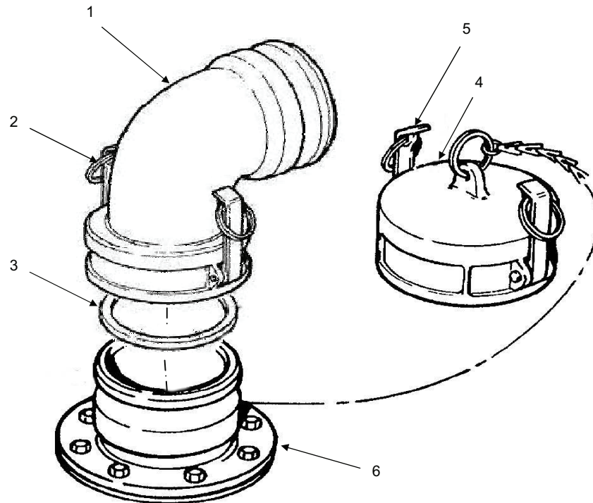
Figure 9. Filler/Discharge Elbow.
