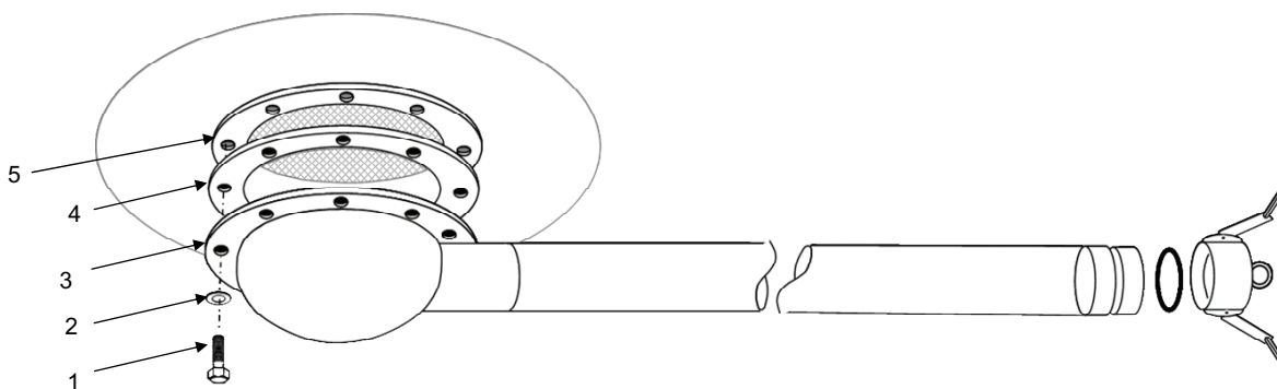
Figure 1. Berm Liner Drain Hose Assembly, Bowl x Cam.
