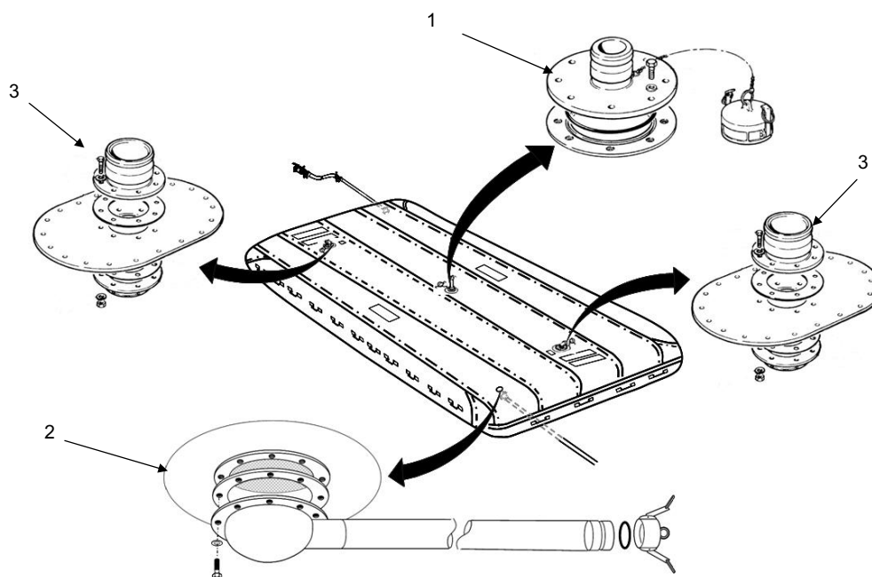
Figure 1. Tank Assembly.
