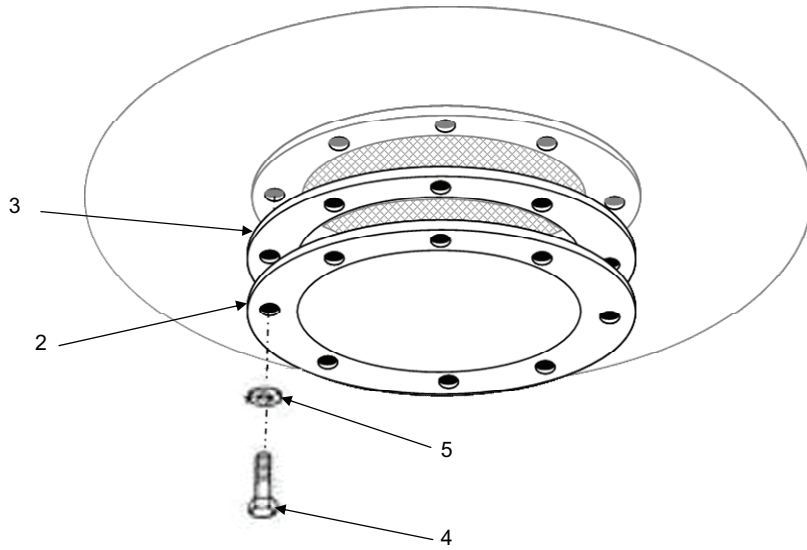
Figure 12. Berm Liner Drain Fitting Assembly.
