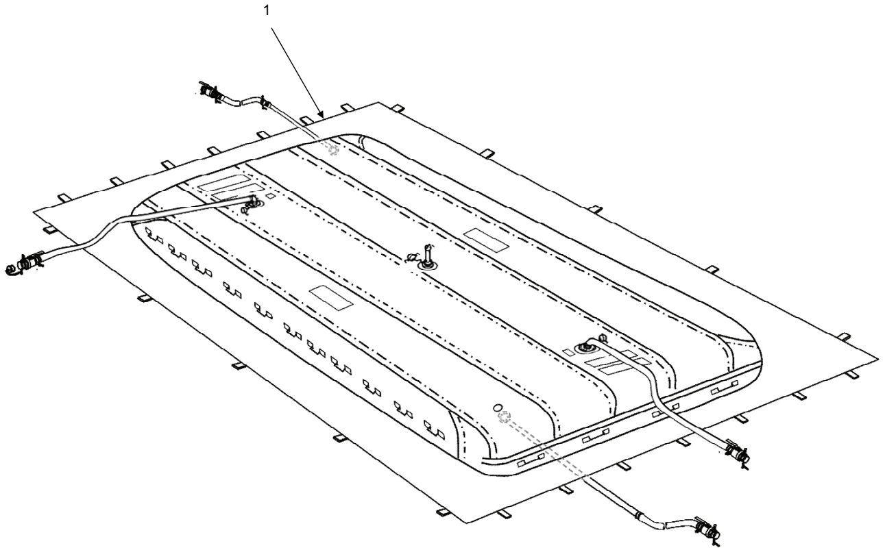
Figure 1. Tank Assembly.
