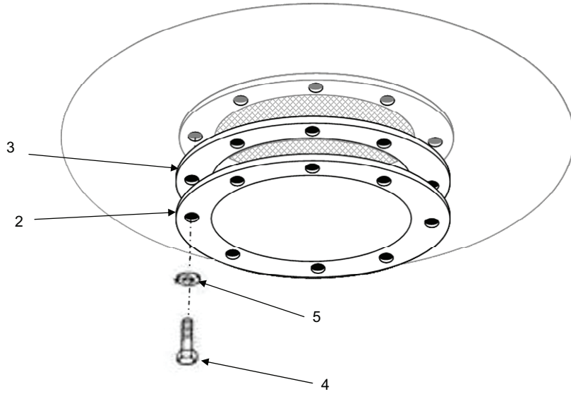
Figure 9. Tank Drain Fitting Assembly.
